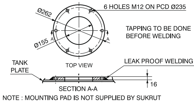
FIG. 4 : MOUNTING PAD
